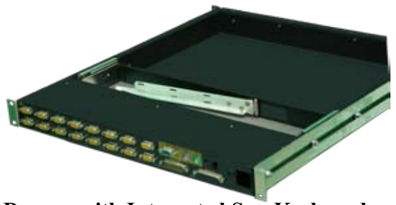
Drawer with Integrated Sun Keyboard and Trackball
